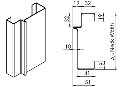
New-Construction Frame Artistic - Artistic Cladding
