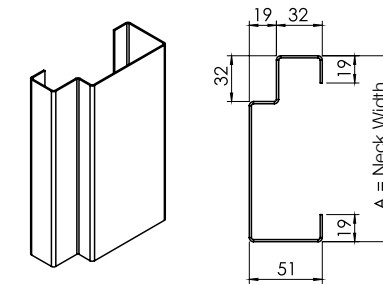
Frame Model C (available with or without "Click On" frame covers)
