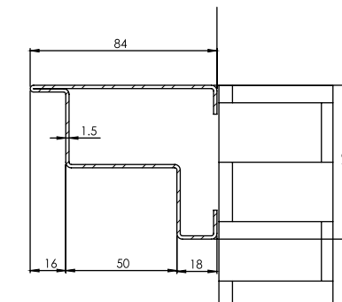
Flush Finish Frame
